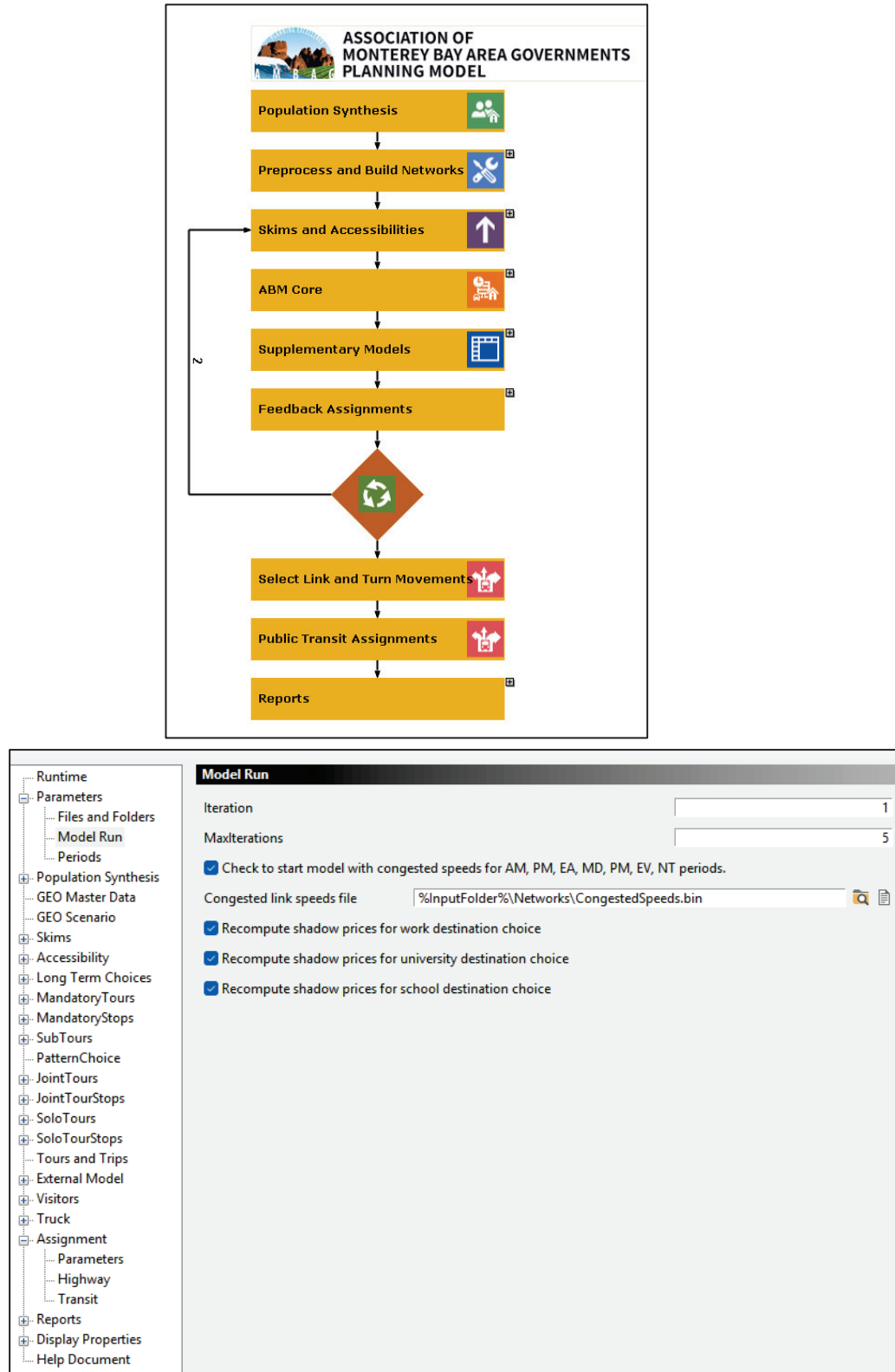
Figure F-1: ABM Flowchart and Model Parameters User Interface
